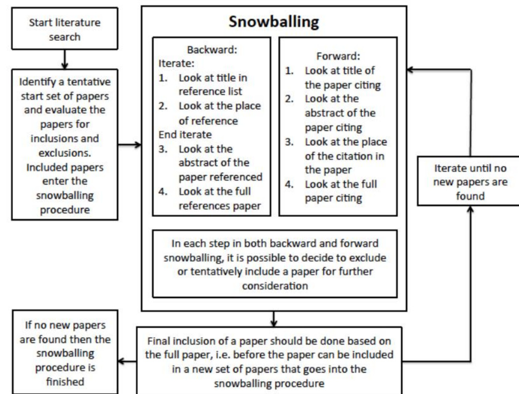
Figure 1. Snowballing procedure.
